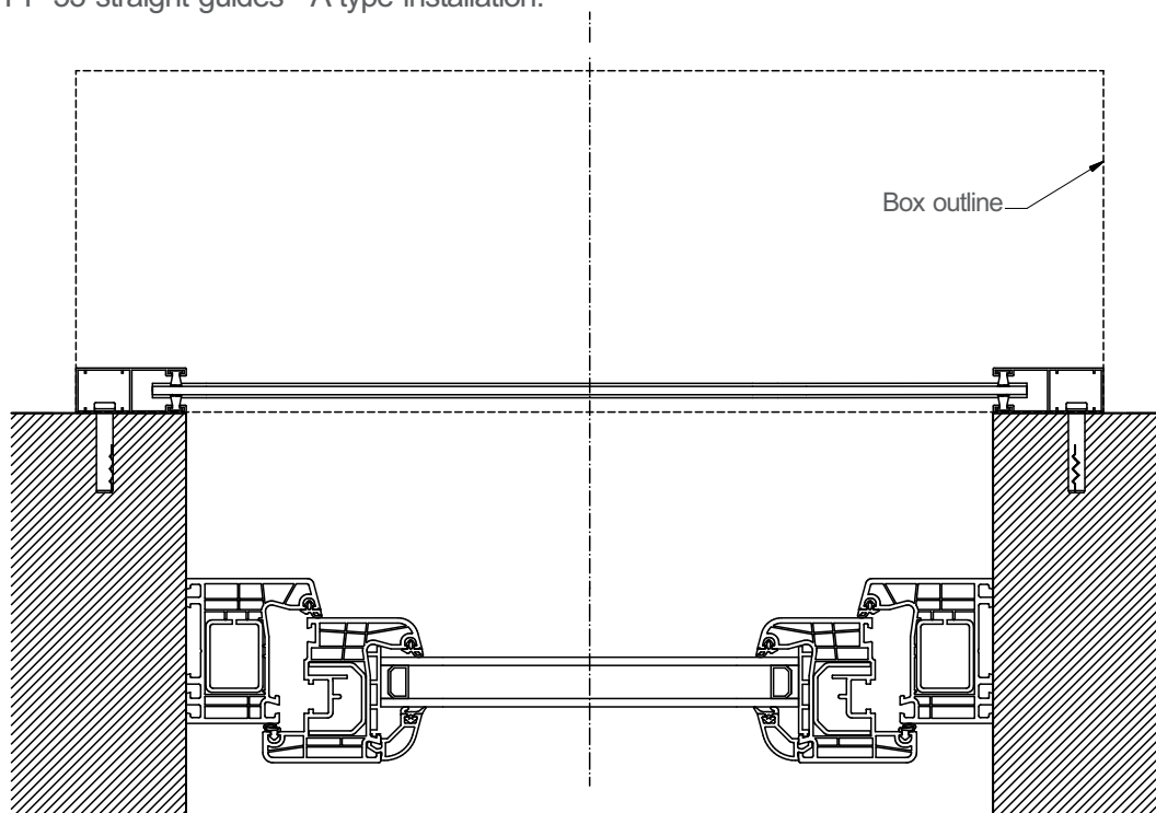
Installation of PP-53 straight guides - A type installation.
