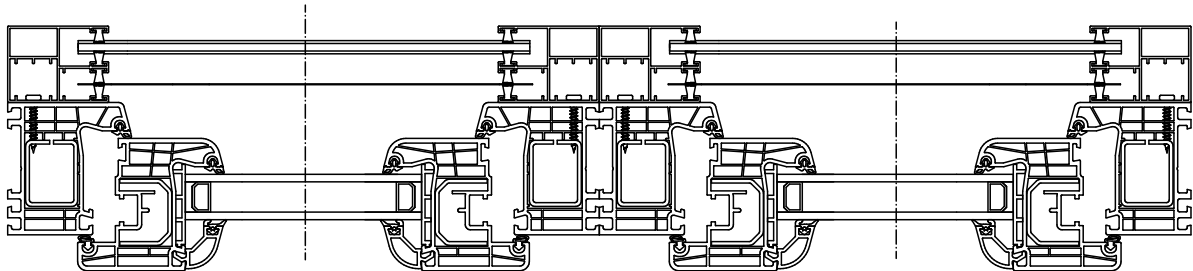
Installation of PPDM-53 guides and PPDM-80 double guide - B type installation.
