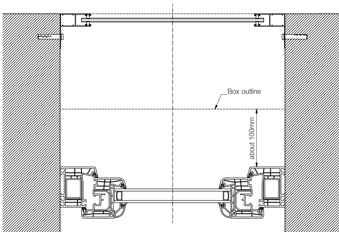
Installation of PK-53 corner guides - C type installation.
