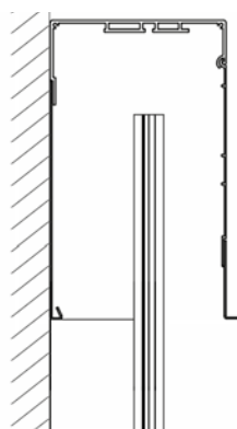
TYP A - Flush-mounted box. Dedicated F-FBR-030 guides.
