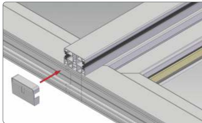
13. If necessary, mount the bottom end caps.
