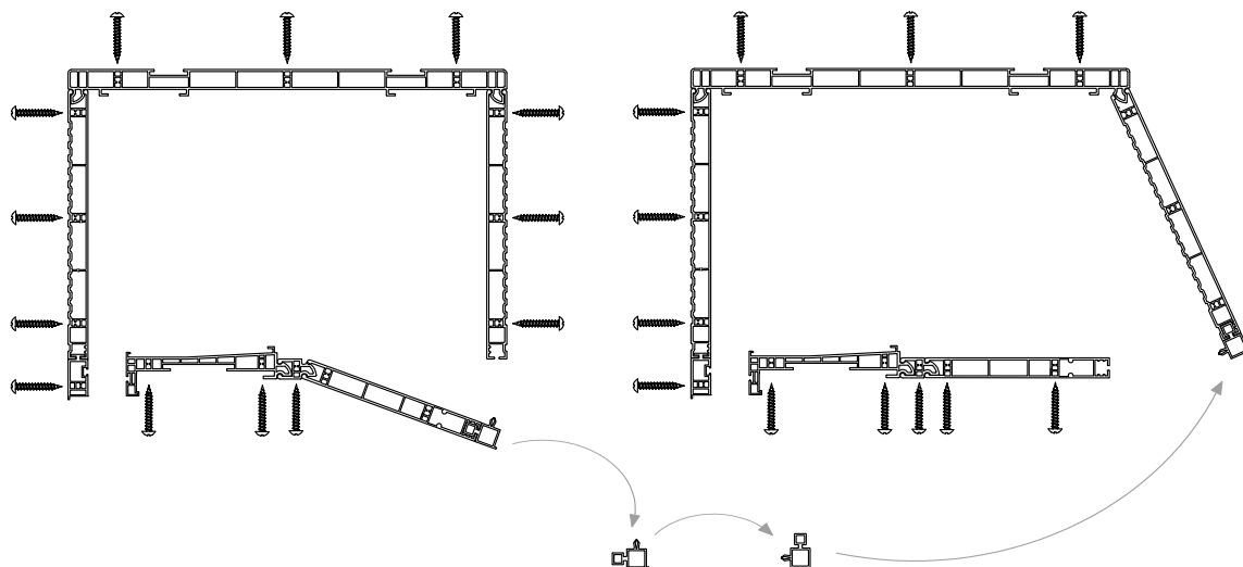
Revision hatches in box 220 without mosquito net
