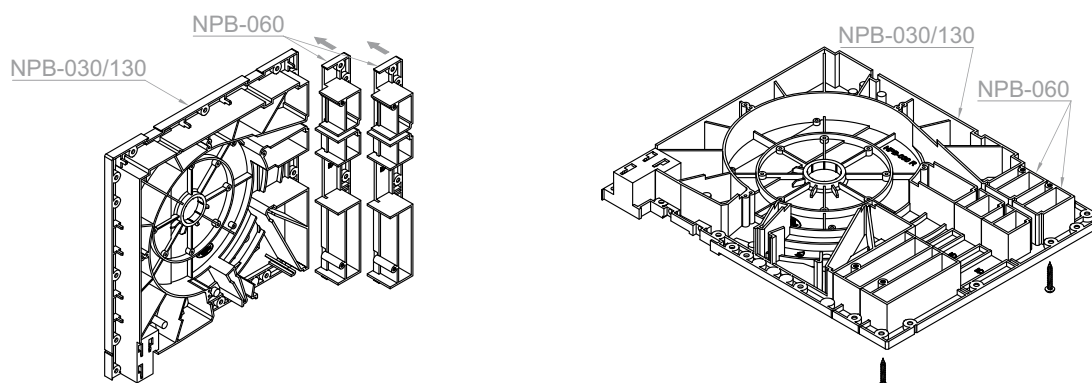
Installation of enlargement +6 2xNPB-060 for BPB 030/130 side
