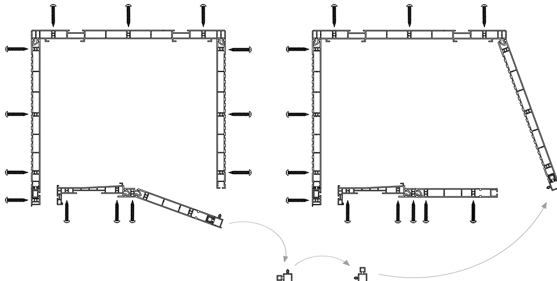
Revision hatches in box 250 without mosquito net
