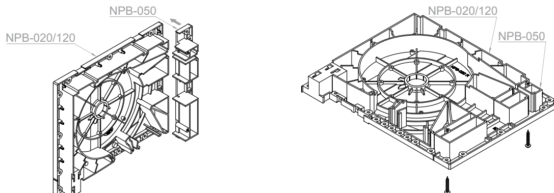
Installation of enlargement + 3 NPB-050 for BPB 020/120 side
