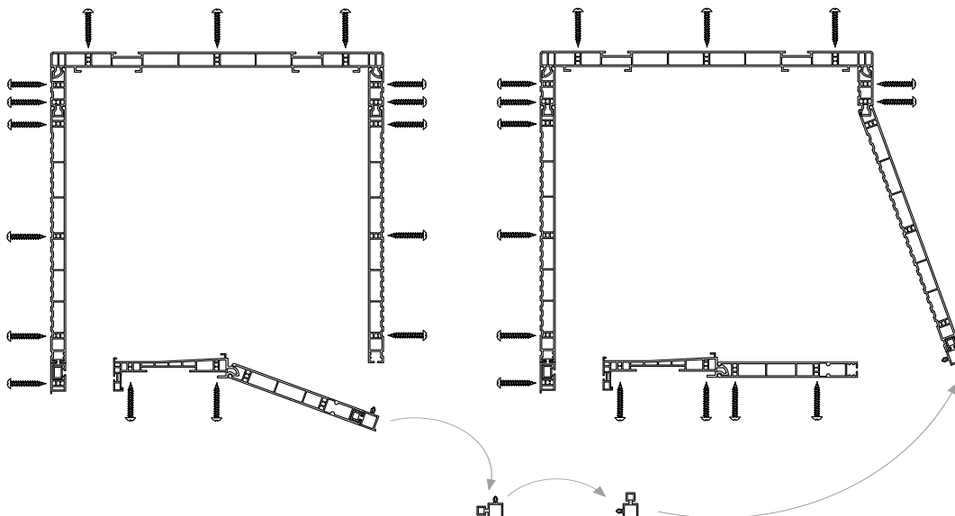
Revision hatches in box 250 with mosquito net
